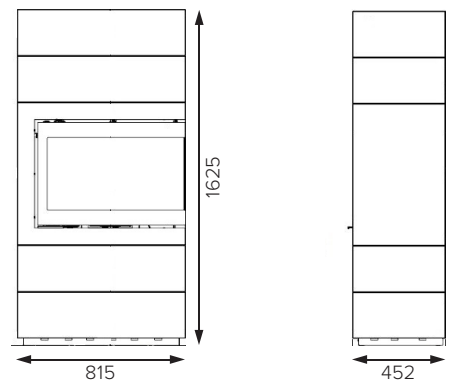
HWAM 5670
